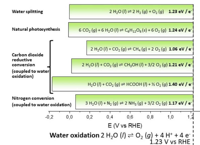
Scheme 1 Schematic representation of the energetic requirements of selected photosynthetic reactions (see eqn (1)–(6) in the main text).
