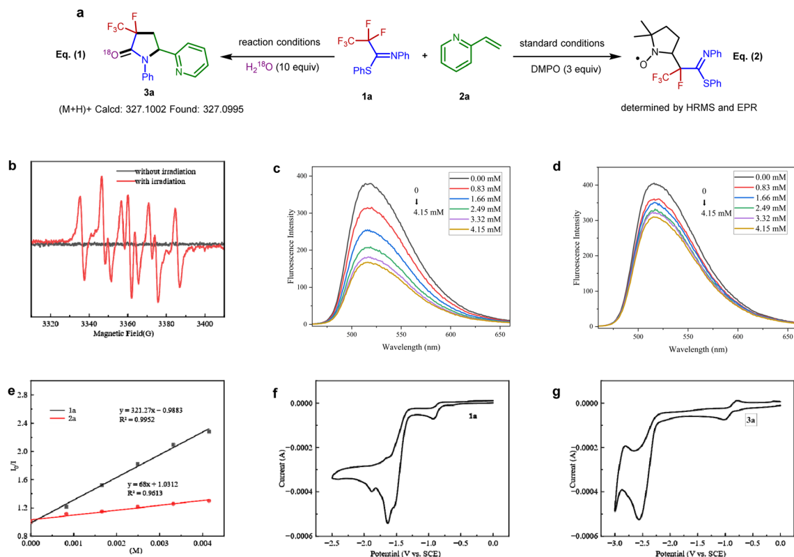
Fig. 3 Mechanistic investigations. (a) 18 O-Labeling experiment and EPR experiment. (b) EPR spectrum. (c) Fluorescence quenching experiments with various concentrations of 1a. (d) Fluorescence quenching experiments with various concentrations of 2a. (e) Stern-Volmer plots with different quenchers. (f) Cyclic voltammograms of 1a. (g) Cyclic voltammograms of 3a.
