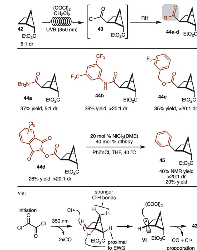
Scheme 5 C–H carboxylation.
