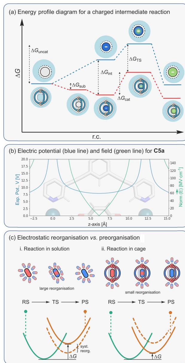
Fig. 13 (a) Energy profile diagram for a reaction with a charged intermediate; (b) electric potential (blue line), V, and field (green line), E, exemplified for a [\text{Pd}_2\text{L}_4]^{4+} cage; (c) electrostatic TS stabilisation via a preorganised microenvironment.
