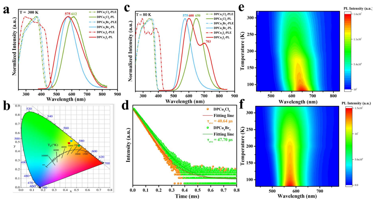
Fig. 2 PL and PLE spectra of \text{DPCu}_4\text{X}_6 ( \text{X} = \text{Cl}, \text{Br}, \text{I} ) SCs measured at (a) 300 K and (c) 80 K (excited at 320 nm, monitored at 600 nm). (b) CIE chromaticity diagram of \text{DPCu}_4\text{X}_6 ( \text{DPCu}_4\text{Cl}_6 , green; \text{DPCu}_4\text{Br}_6 , red; \text{DPCu}_4\text{I}_6 , blue). (d) The RT-TRPL spectra of \text{DPCu}_4\text{X}_6 ( \text{X} = \text{Cl}, \text{Br} ) SCs probed at 600 nm. Temperature-dependent PL spectra of (e) \text{DPCu}_4\text{Cl}_6 and (f) \text{DPCu}_4\text{Br}_6 .
