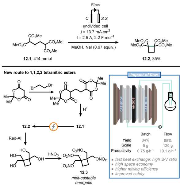
Fig. 12 Flow electrochemistry facilitates the safe scale-up of a promising melt-castable energetic intermediate. C: graphite electrode; S. S: stainless steel electrode.
