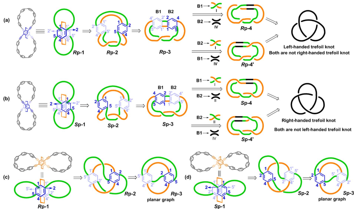
Fig. 2 Topological analyses: (a and b) representative topological transformations of R_p - bis-pm-TC and S_p - bis-pm-TC into the left- and right-handed trefoil knot graphs, respectively. (c and d) Representative topological transformation of R_p - bis-po-CC and S_p - bis-po-CC into the planar graphs.
