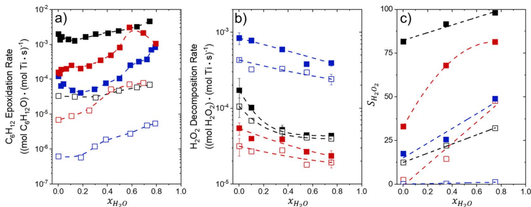
Fig. 1 Turnover rates for (a) C_6H_{12} epoxidation to form C_6H_{12}O (1 mM C_6H_{12} , 10 mM H_2O_2 , 313 K), (b) H_2O_2 decomposition (1 mM H_2O_2 , 10 mM C_6H_{12} , 313 K) and (c) H_2O_2 selectivities for epoxidation (1 mM C_6H_{12} , 10 mM H_2O_2 , 313 K) as a function of H_2O mole fraction in mixtures of CH_3CN (■, □), CH_3OH (■, □), and C_4H_6O_2 (■, □) with H_2O over Ti-BEA-OH (solid points) and Ti-BEA-F (hollow points). The furthest left data points represent x_{H_2O} = 0.002 , which comes from the aqueous H_2O_2 reagent solution (39 mM).
