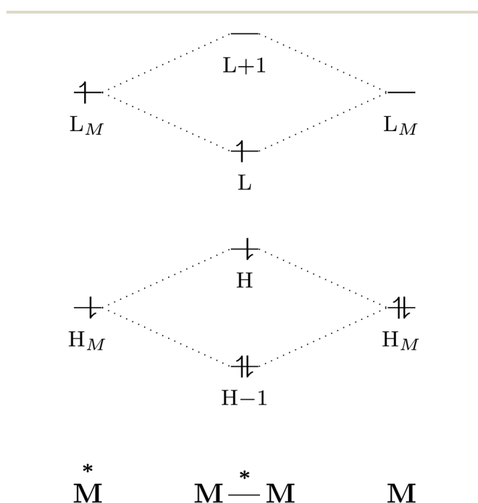
Fig. 1 Simplified molecular orbital diagram describing the formation of an excimer from molecular orbitals of the monomers as described in eqn (1). "H" and "L" refer to the highest occupied and lowest unoccupied molecular orbitals, respectively; based on similar examples in ref. 1 and 5–7.
