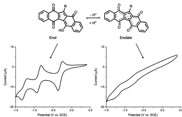
Fig. 5 Cyclic voltammetry of KuQEt in CH_2Cl_2/TBAP\ 0.1\ M (left) and DMF/TBAP\ 0.1\ M (right). WE: glassy carbon, RE: saturated calomel electrode, CE: platinum wire. Adapted from ref. 29. Copyright 2021 The Authors. Published by American Chemical Society.
