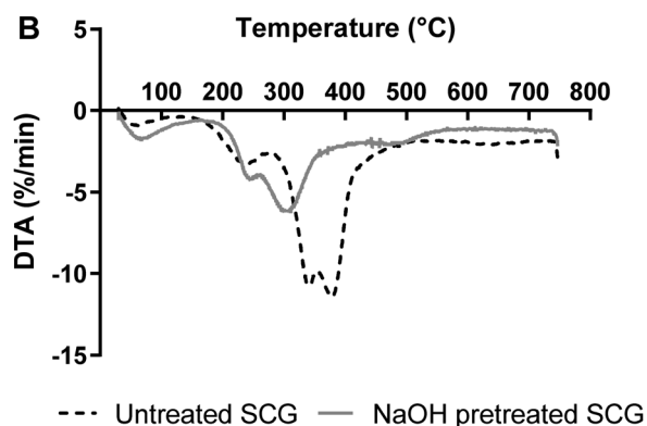
Fig. 2 TGA (A) and DTA (B) curves obtained for pretreated and untreated SCG.
