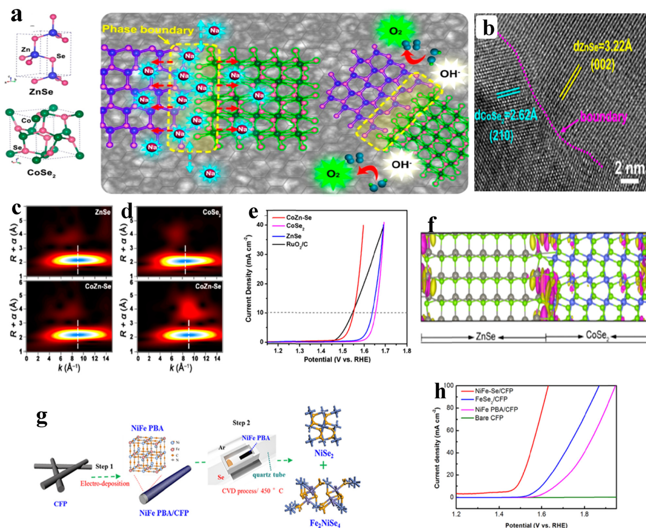
Fig. 12 (a) Schematic diagram of the phase boundary effect in CoZn–Se; (b) HR-TEM image showing the boundary between CoSe and ZnSe; (c) and (d) k_2 -weighted K-edge EXAFS signals of Zn and Co for ZnSe and CoZn–Se, respectively; (e) LSV curves of CoZn–Se, CoSe, ZnSe and RuO 2 ; (f) charge density profile at the phase boundary between CoSe and ZnSe; (g) schematic illustration of NiFe–Se/CFP synthesis; (h) LSV polarization results of NiFe–Se, FeSe 2 and NiFe PBA over CFP. Reprinted with permission from ref. 90. Copyright (2021) American Chemical Society (ACS).
