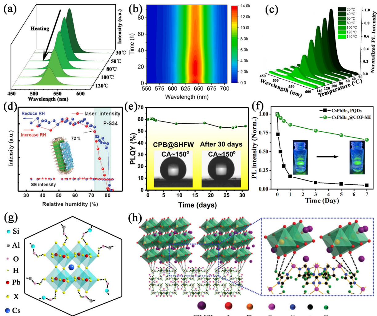
Fig. 15 (a) Temperature-dependent PL spectra for \text{CsPbBr}_3 @zeolite. Adapted from ref. 113 with permission. Copyright 2021, Wiley-VCH. (b) Color-coded contour maps showing the time-dependent emission spectra of \text{CsPbBr}_3 @HP-UiO-66. Adapted from ref. 131 with permission. Copyright 2021, Elsevier. (c) Temperature-dependent PL spectra of \text{CsPbBr}_3 @Ce-MOF@ \text{SiO}_2 composites. Reproduced from ref. 148 with permission. Copyright 2022, Elsevier. (d) Lasing and spontaneous emission of \text{CsPbBr}_3 @SAPO-34 as a function of relative humidity. Adapted from ref. 111 with permission. Copyright 2020, Royal Society of Chemistry. (e) Time-dependent PLQY of \text{CsPbBr}_3 @SHFW composite powders in water. Adapted from ref. 150 with permission. Copyright 2019, American Chemical Society. (f) Time-dependent normalized PL intensity of \text{CsPbBr}_3 and \text{CsPbBr}_3 @COF-SH in water. Adapted from ref. 144 with permission. Copyright 2023, Elsevier. (g) Schematic illustration of \text{CsPbBr}_3 restricted in zeolite, showing H-bonding interactions between zeolite and \text{CsPbBr}_3 . Reproduced from ref. 113 with permission. Copyright 2021, Wiley-VCH. (h) Schematic illustration of the interaction between \text{MAPbI}_3 and ZIF-8. Adapted from ref. 151 with permission. Copyright 2018, Royal Society of Chemistry.
