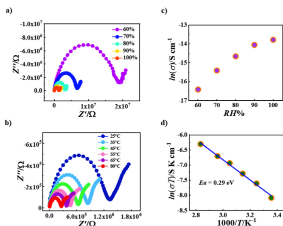
Fig. 6 Nyquist plots for R -1 at 25\text{ }^\circ\text{C} under different relative humidity (RH) levels (a). Nyquist plots for R -1 at different temperatures under 100% relative humidity (RH) (b). Plots of proton conductivity vs. RH for R -1 at 25\text{ }^\circ\text{C} (c). Plots of \ln(\sigma T) vs. 1000/T for R -1 under 100% relative humidity (RH) (d).
