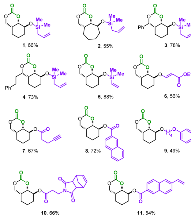
Scheme 2 General synthetic scheme for the functionalized bicyclic six-membered cyclic carbonate monomers 1–11 derived from precursor 6MCCs A–D. FG-X stands for the coupling agent used to produce the functionalized bicyclic 6MCC.
