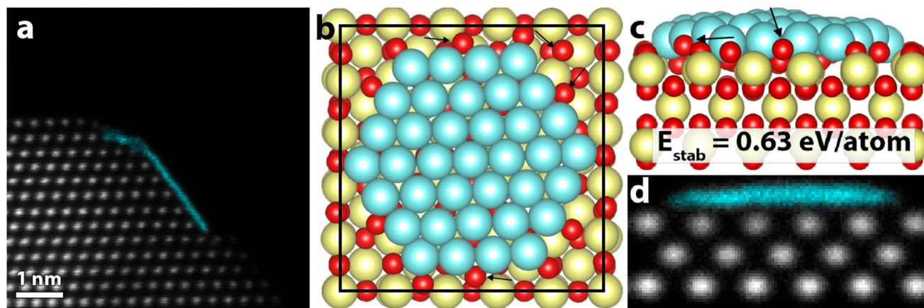
Fig. 4 (a) HAADF-STEM image of the final 2D structure. (b) Relaxed model of a Pt(111) raft on a CeO 2 (100) surface. (c) Side view of (b). Black arrows point to a few examples of large structural relaxation in the CeO 2 surface oxygen anions. (d) STEM simulation of the structural model in (b) and (c), showing a similar signature as the experimental observation in (a). False color STEM image: columns identified as Pt, based on the local lattice spacing and image intensity, are plotted in turquoise (grayscale version in Fig. S10†).
