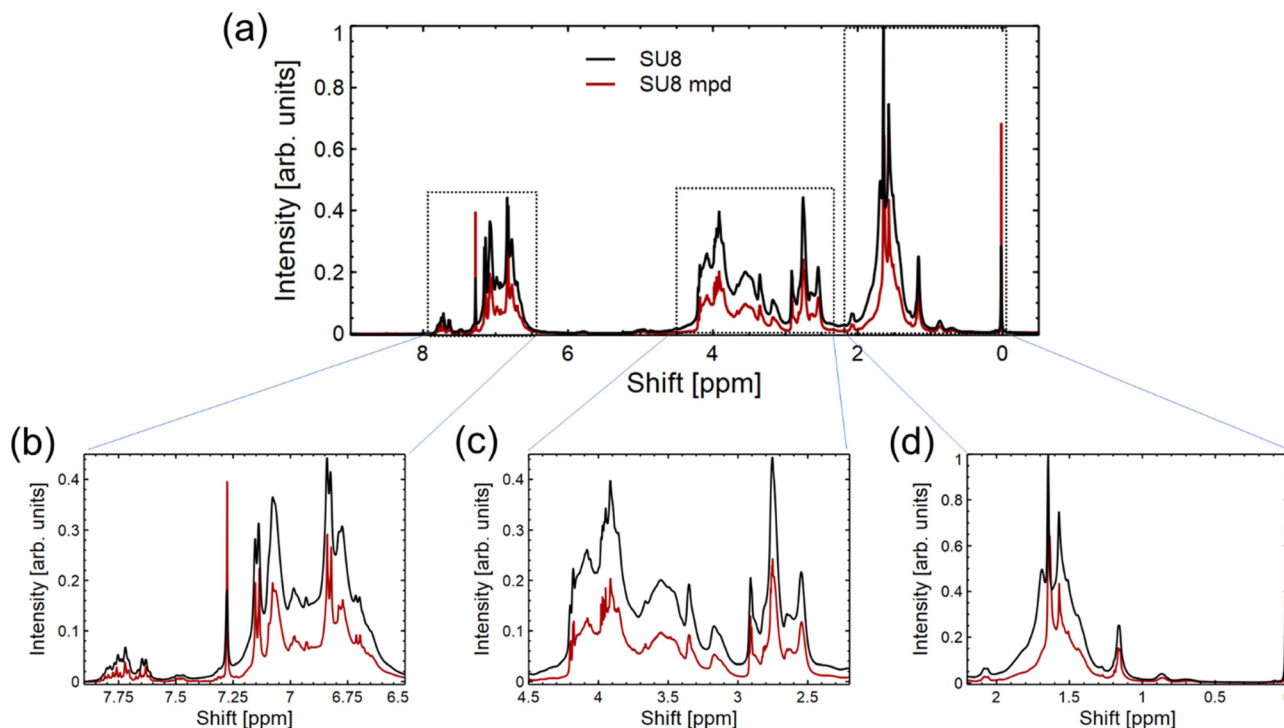
Fig. 4 1 H-NMR analysis of the SU8- m -PD conjugate. (a) Provides a full view of the entire spectrum. Region-specific magnifications further elucidate the interactions: (b) emphasizing the 6.5–8 ppm range, which is dominated by aromatic proton resonances, indicative of the SU8 and m -PD aromatic structures. (c) The 2.25–4.5 ppm region, highlighting potential transitional groups and intermediates; and (d) focusing on the 0–2.25 ppm range, predominantly showcasing aliphatic proton environments.
