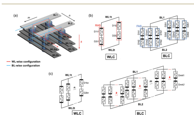
Fig. 4 The vertical 2 \times 2 crossbar array structure. (a) The three-layered structure and its configurations. The equivalent circuit of configurations when (b) n = 2 , m = 2 , and k = 3 , and (c) for a larger size. The high parallel FAS gates indicated in blue dotted boxes can be achieved in the BLC. The number of possible circuits in the BLC is dependent on k .
