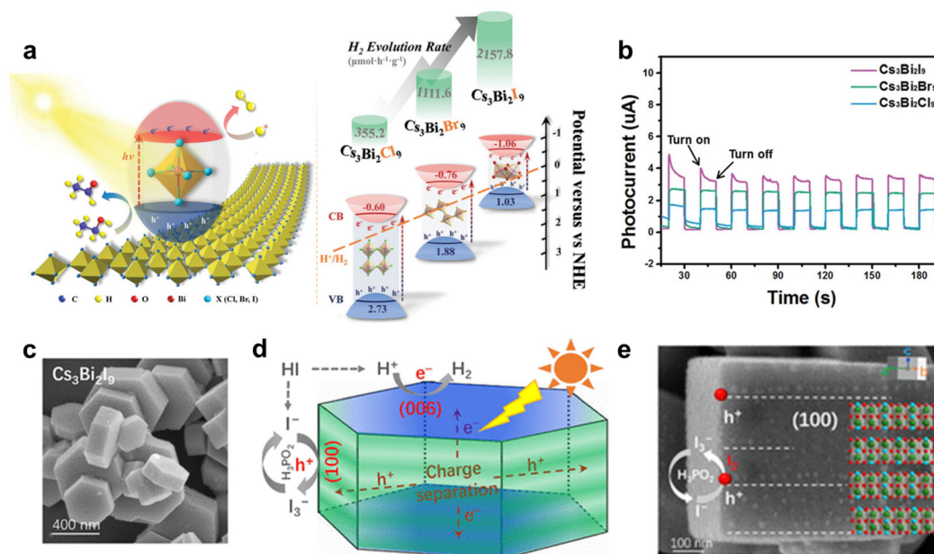
Fig. 6 (a) Schematic mechanism of H 2 evolution by Cs 3 Bi 2 X 9 nanosheets in ethanol. (b) Transient photocurrent responses of the photocatalysts. Reproduced with permission from ref. 143. Copyright 2022 Wiley-VCH. (c) Morphology and crystalline structure of Cs 3 Bi 2 I 9 hexagonal prisms. (d) H 2 production process and anisotropic charge transfer to the different redox facets. (e) SEM image of the photocatalysts after reaction for 8 h. Reproduced with permission from ref. 94. Copyright 2022 American Chemical Society.
