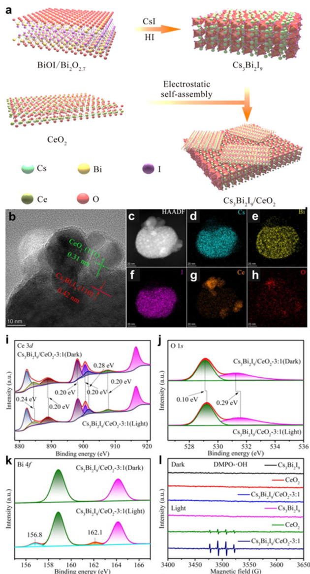
Fig. 5 (a) The preparation of Cs 3 Bi 2 I 9 nanosheets and the self-assembly between Cs 3 Bi 2 I 9 and CeO 2 nanosheets. (b) HRTEM image of Cs 3 Bi 2 I 9 /CeO 2 -3 : 1 assembly. (c–h) High-angle annular dark field (HAADF) image and elemental mapping images of Cs 3 Bi 2 I 9 /CeO 2 -3 : 1. (i–k) High-resolution XPS spectra of (i) Ce 3d, (j) O 1s and (k) Bi 4f for Cs 3 Bi 2 I 9 /CeO 2 -3 : 1 under dark and light excitation. (l) ESR spectra of Cs 3 Bi 2 I 9 , CeO 2 and Cs 3 Bi 2 I 9 /CeO 2 -3 : 1 with DMPO as the radical trap. Reproduced with permission from ref. 104. Copyright 2021 Science Press and Dalian Institute of Chemical Physics, Chinese Academy of Sciences.
