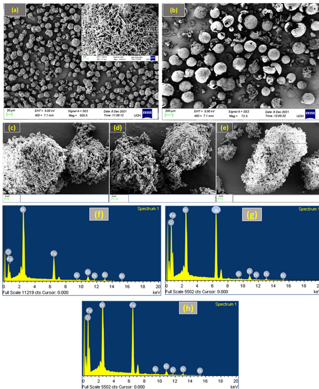
Fig. 2 FE-SEM images of (a) pure BFO, (b) pure Fe 2 O 3 , (c) BFO10, (d) BFO20, and (e) BFO30, and EDAX spectra of (f) BFO10, (g) BFO20, and (h) BFO30.
