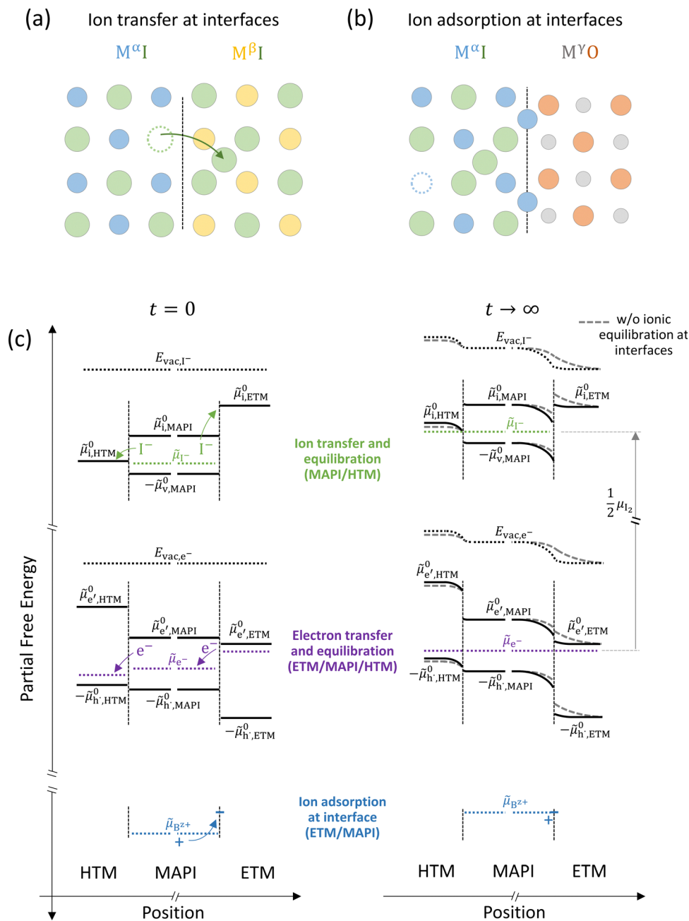
Fig. 7 (a) Ionic equilibration between two metal iodide phases M^{\alpha}I and M^{\beta}I , where transfer of I^{-} from M^{\alpha}I to M^{\beta}I increases the concentration of V_{M}^{\bullet} on the left side and of I_{i}^{-} on the right side of the interface giving rise to an interfacial equilibrium space charge ( \Delta\mu_{I^{-}} \neq 0 and different standard potentials of defect formations in the two phases are assumed). (b) Metal cation adsorption from a metal iodide M^{\alpha}I on the interface of a second phase (here an oxide M^{\gamma}O ) induces a space charge region where positive defects are depleted and the concentration of negative defects (here V_{M}^{\bullet} and I_{i}^{-} ) is increased. (c) Example of an extended ionic and electronic energy diagram of a MAPI solar cell in the dark at equilibrium where the interfaces are highlighted. Ion transfer (here I^{-} ) and ion adsorption (here B^{z+} adsorbed at the MAPI/ETM interface, e.g. Pb^{2+} adsorbed on TiO_2 surface 47 ) can have significant repercussion on the chemical and electrostatic situation at interfaces. The situations upon contact ( t = 0 ) and after equilibration ( t \rightarrow \infty ) are shown. In the right diagram, dashed lines indicate the situation where ionic equilibration with contact materials is not considered.
