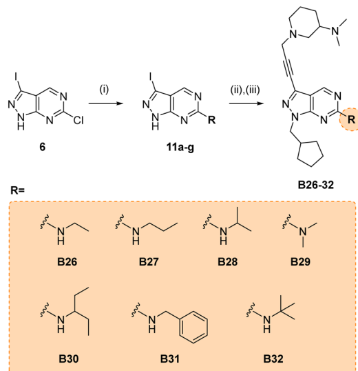
Scheme 5 Synthesis of B26-32 . Reagents and conditions: (i) alkyamine, \text{THF} , 150^\circ\text{C} , \mu\text{w} , 60 min, 46–73%; (ii) (iodomethyl) cyclopentane, \text{NaH} , \text{DMF} , 150^\circ\text{C} , \mu\text{w} , 85 min, 37–68%; (iii) 10n , \text{Pd}(\text{PPh}_3)_2\text{Cl}_2 , \text{CuI} , \text{TEA} , \text{THF} , 70^\circ\text{C} , \mu\text{w} , 2 h, 26–59%.
