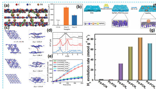
Fig. 9 (a) Conceptual illustration of a Pd/g-CN hybrid with the interlayer intercalation and surface anchor of Pd atom. (b) Photocatalytic H 2 evolution activities of CN-NS, Pd/g-CN, and Pt/g-CN. 51 (c) Possible coordination approaches of Pd SAs with DNUCN and the corresponding adsorption energy of Pd SAs at different anchoring sites. (d) R space of 0.16%Pd/DN-UCN 0.50 . (e) Photocatalytic H 2 evolution activity of Pd/CN hetero-junctions obtained by different CN nanosheets. 52 (f) Synthesis and structural characterization of Pd/PCNx catalysts. (g) Comparison of H 2 evolution rate for these as-prepared samples under simulated sunlight. 53
