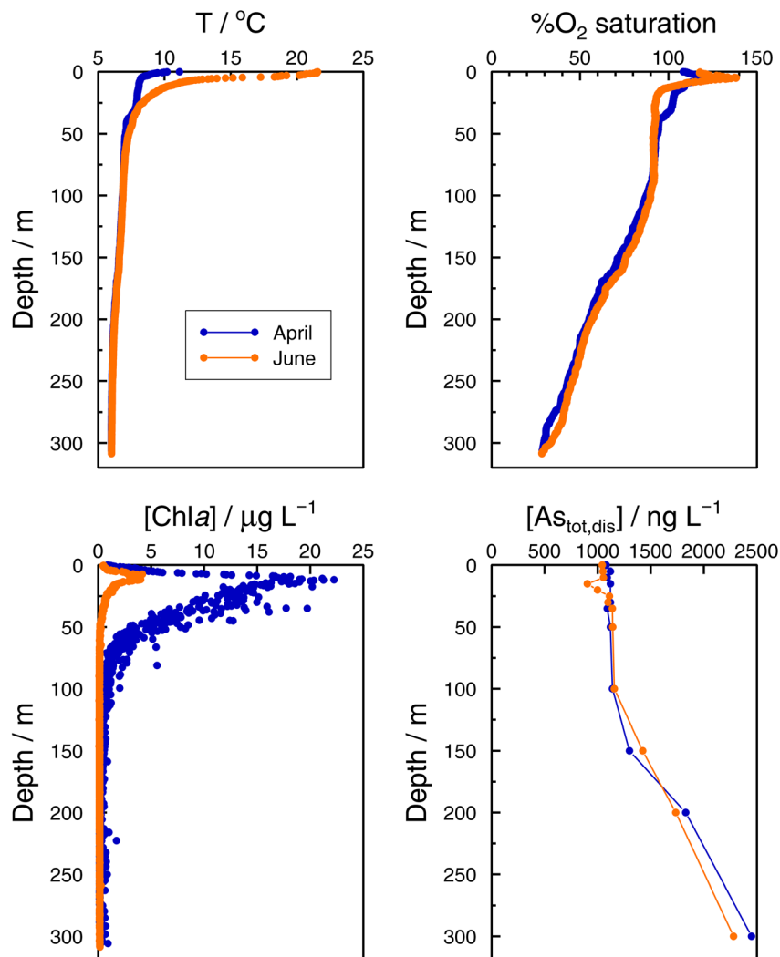
Fig. 5 Vertical profiles of temperature, percentage of O 2 saturation, chlorophyll a, and total dissolved arsenic, As total,dis in the Grand Lac (point SHL2) in April (blue) and June (orange) 2021.
