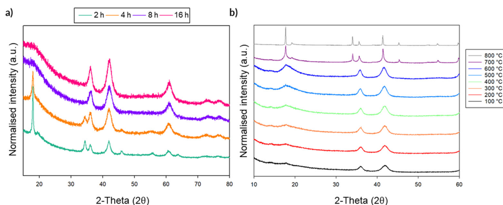
Fig. 12 (a) XRD of Li 2 SnO 3 with increasing mill time. Conversion to DRS occurs at ~8 h (b) Plot showing the changes in XRD pattern with increasing temperature, showing the transformation from DRS to layered on heating. (Cu K \alpha ).
