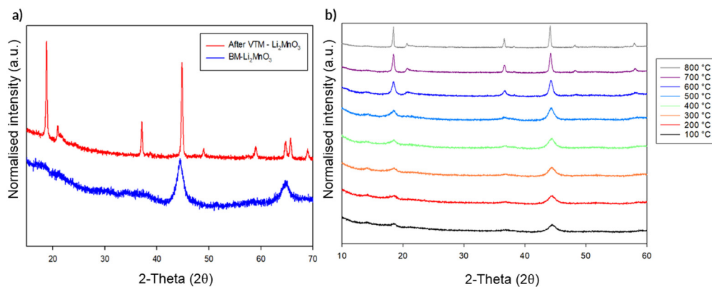
Fig. 11 (a) XRD of BM-Li 2 MnO 3 sample before (DRS phase) and after VT-XRD (layered phase) (b) VT-XRD experiment in the region of 100–800 °C showing the change in the relative intensity of peaks with increasing temperature indicating a transformation from DRS to layered on heating. (Cu K \alpha ).
