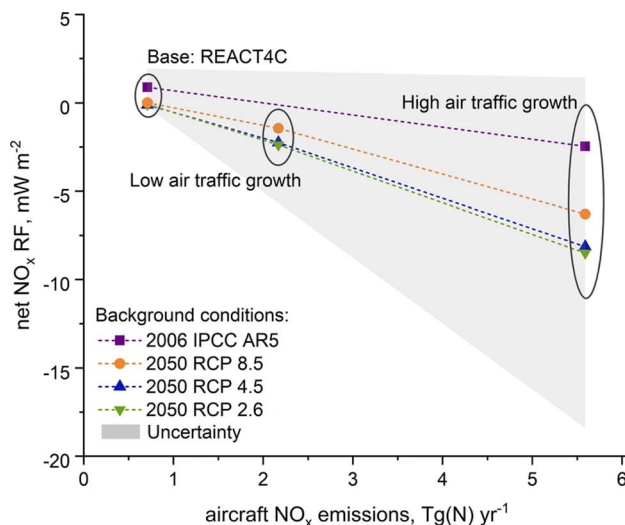
Fig. 15 Aviation net NO x radiative forcing (RF) (the sum of the short-term positive O 3 RF perturbation and the negative RF terms caused by a reduction in CH 4 lifetime), by aviation NO x emission rate according to a range of background emission scenarios. Aviation net NO x RF systematically decreases with increasing NO x emissions from aviation, showing a variation according to the background surface emissions, with high mitigation (RCP 2.6) having a smaller (or ‘more negative’) at larger emission rates) aviation net NO x RF than, lower mitigation scenarios (RCP 4.5, RCP 8.5) for the same aviation NO x emission. Overall uncertainties are indicated by the grey shading, which is one standard deviation (68% confidence interval). From Skowron et al. (2021). 129
