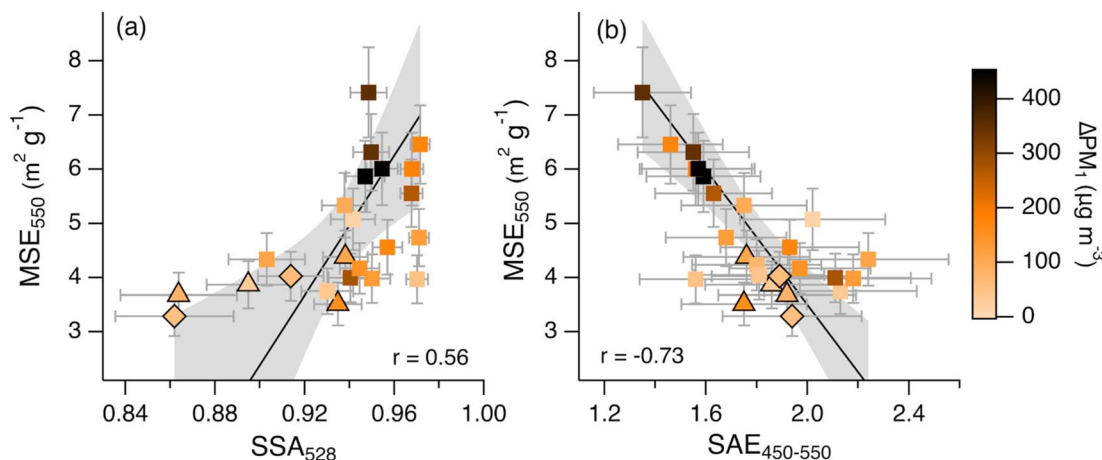
Fig. 6 Mass scattering efficiency (MSE; \sigma_{\text{scat}}/\text{PM}_1 ) at 550 nm plotted as a function of (a) single scattering albedo (SSA) at 528 nm, and (b) the scattering Ångström exponent (SAE). Each event is colored by the absolute \text{PM}_1 enhancement ( \Delta\text{PM}_1 ). Error bars show precision uncertainty. Data are fit with reduced major axis (RMA) regressions with shading representing the 95% confidence interval of the fits. Events are shaped according to their origin in the same way as in Fig. 3. Pearson's correlation coefficients ( r ) are shown for the plotted relationships. The r values for MSE vs. \Delta\text{PM}_1 and SAE vs. \Delta\text{PM}_1 are 0.69 and -0.44 , respectively.
