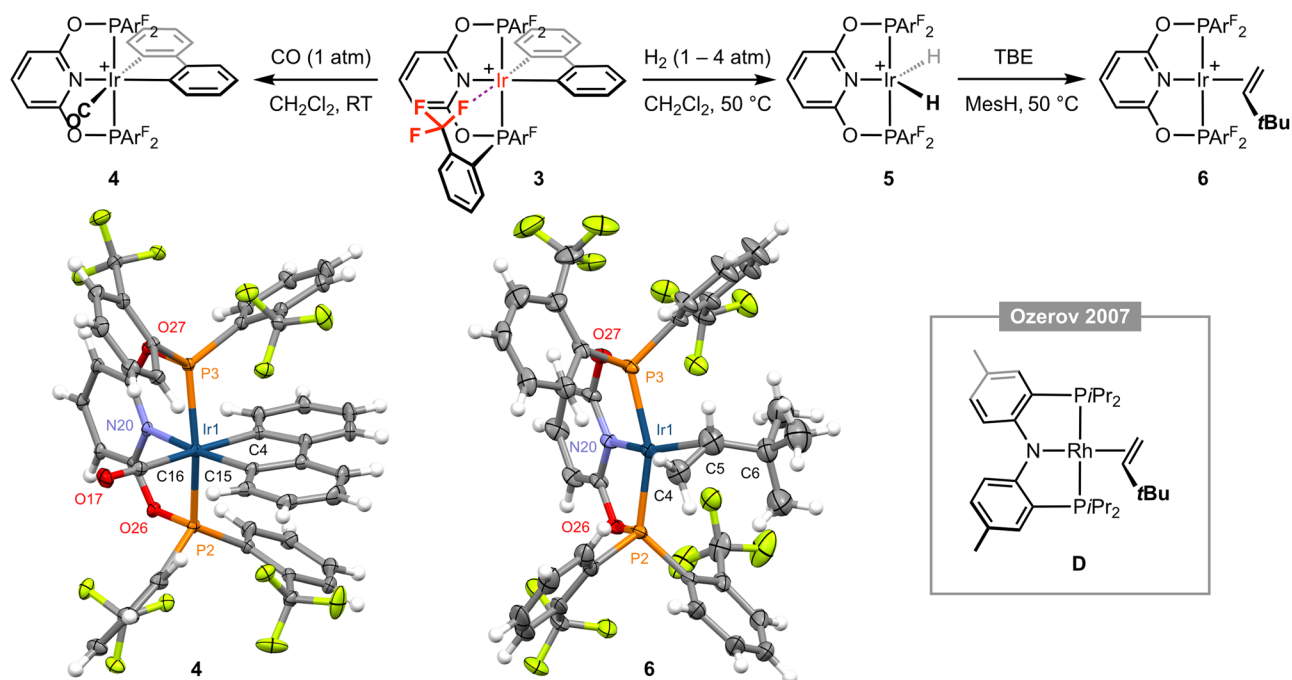
Fig. 3 Reactivity of complex 3; MesH = mesitylene and [BAr^f_4]^- counter ions omitted for clarity. Solid-state structures of 4 and 6 drawn with thermal ellipsoids at 30% probability and without solvent molecules. Selected metal-based bond lengths (Å) and angles (°): 4, Ir1–P2, 2.3300(7); Ir1–P3, 2.3243(7); Ir1–N20, 2.102(2); Ir1–C4, 2.092(3); Ir1–C15, 2.072(3); Ir1–C16, 1.958(3); C16–O17, 1.123(4); P2–Ir1–P3, 159.85(2); N20–Ir1–C15, 171.25(10); C4–Ir1–C16, 177.09(11); 6, Ir1–P2, 2.2657(11); Ir1–P3, 2.2704(12); Ir1–N20, 2.058(4); Ir1–Cnt(C4,C5), 2.110(12); C4–C5, 1.304(12); P2–Ir1–P3, 156.46(5); N20–Ir1–Cnt(C4,C5), 175.3(4); C4–C5–C6, 130.6(10); D, Rh–Cnt(C=C), 2.051(3); C=C, 1.360(10); N–Rh–Cnt(C=C), 174.27(14); C=C–C, 127.7(5). 15 Cnt = centroid.
