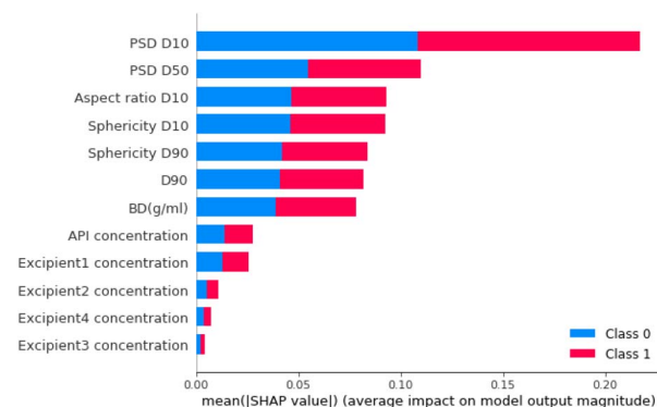
Fig. 14 Feature importance analysis for the RF model in step 1. The features are ranked based on their absolute mean SHAP score. The impact of each feature on each class is represented using colours and hence, the impact of the prediction on the output non-free flowing is represented in blue and the impact of the output free flowing is represented in red.
