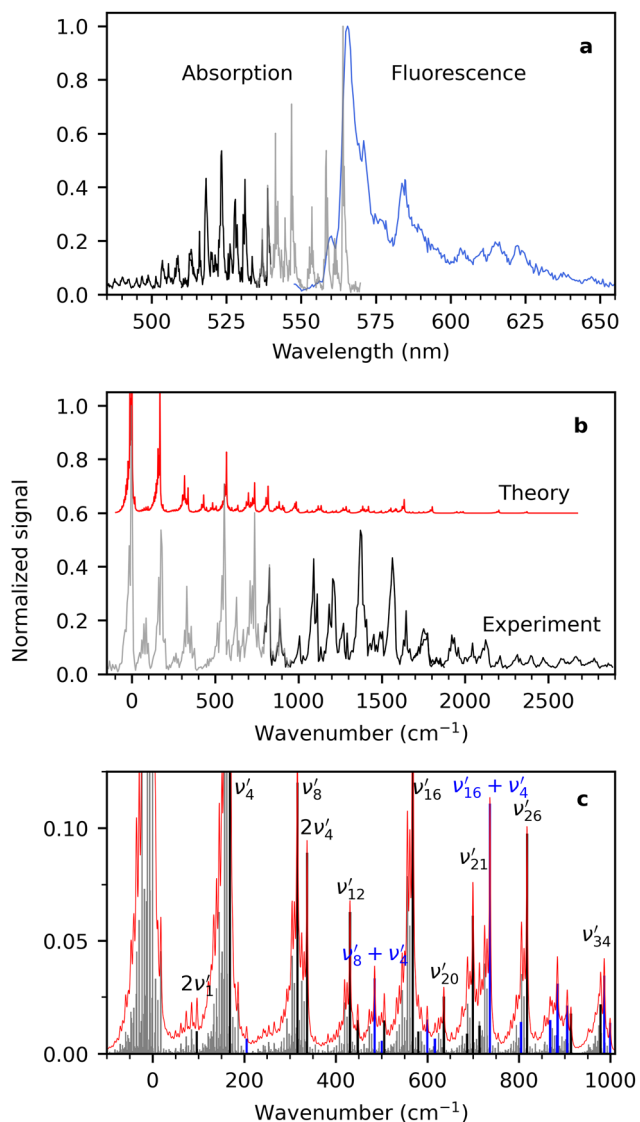
Fig. 2 (a) Fluorescence-excitation (absorption) and dispersed-fluorescence spectra of \text{R}^- measured at 100 K. The former was measured using two different notch filters: the grey spectrum (535–570 nm) was obtained from collecting emitted photons with wavelengths above 600 nm and the black spectrum (485–540 nm) from photons with wavelengths above 550 nm. The dispersed fluorescence spectrum is shown in blue. The excitation wavelength was 531.3 nm, and the laser power was <0.3 mW. (b) Comparison of experimental (black and grey) and simulated (red) absorption spectra at 100 K. The maximum of each spectrum is used as the zero point for the energy axis. The simulated spectrum is shown with an offset to improve readability. (c) All transitions (grey) contributing to the total simulated absorption spectrum (red). The black transitions are significant transitions from the vibrational ground state ( 0'' ) to the final state indicated by the labels. Blue transitions involve combinations of two or more of the black transitions. Assignments of additional transitions are shown in Fig. S2 in the ESI†
