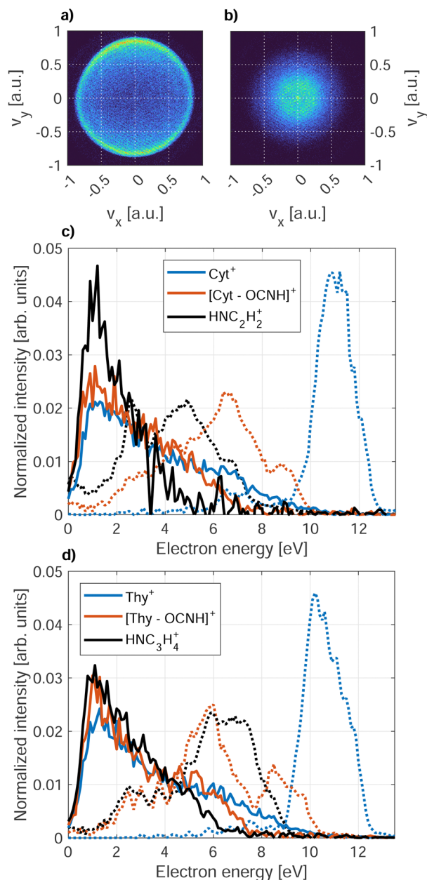
Fig. 7 VMIs of electrons in coincidence with Cyt + recorded for (a) direct photoionization of effusive Cyt ( h\nu = 20.6 eV) and (b) Penning ionization of Cyt in HNDs ( h\nu = 21.6 eV). Panels (c) and (d) show PIES ( h\nu = 21.6 eV) of HND-doped Cyt and Thy, respectively, for the three main electron-ion coincidence channels (solid lines). The dotted lines show the corresponding electron spectra of effusive Cyt and Thy ( h\nu = 20.6 eV).
