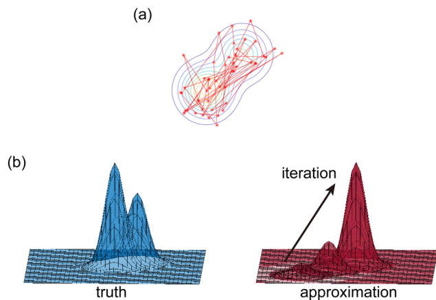
Fig. 2 Illustration of two Bayesian methods. (a) Hamiltonian Monte Carlo (HMC). The HMC method generates samples of B-CRNN weights by sequentially exploring the posterior distribution of the weights. (b) The variational inference method (VI). The VI method approximates the posterior distribution of the weights with a proxy distribution (normally Gaussian), by iteratively minimizing the Kullback–Leibler divergence between the proxy distribution and the true posterior distribution.
