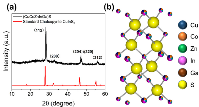
Fig. 1 Figure of (a) powder X-ray diffraction pattern of thin film (CoCuZnGa)S with reference to standard chalcopyrite (CuInS 2 , ICSD: 66865). (b) The crystal structure of HE chalcopyrite ( a = b = 5.52 , c = 11.13 , \alpha = \beta = \gamma = 90^\circ ).
