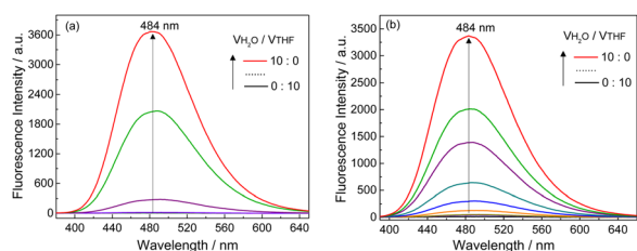
Fig. 4 Fluorescence spectra of (a) \text{L-1} and (b) \text{Ag}^+-\text{L-1} in \text{H}_2\text{O}/\text{THF} mixtures with increasing volume fractions of \text{H}_2\text{O} . \lambda_{\text{ex}} = 350 \text{ nm} , [\text{L-1}] = [\text{Ag}^+-\text{L-1}] = 25 \mu\text{M} .
