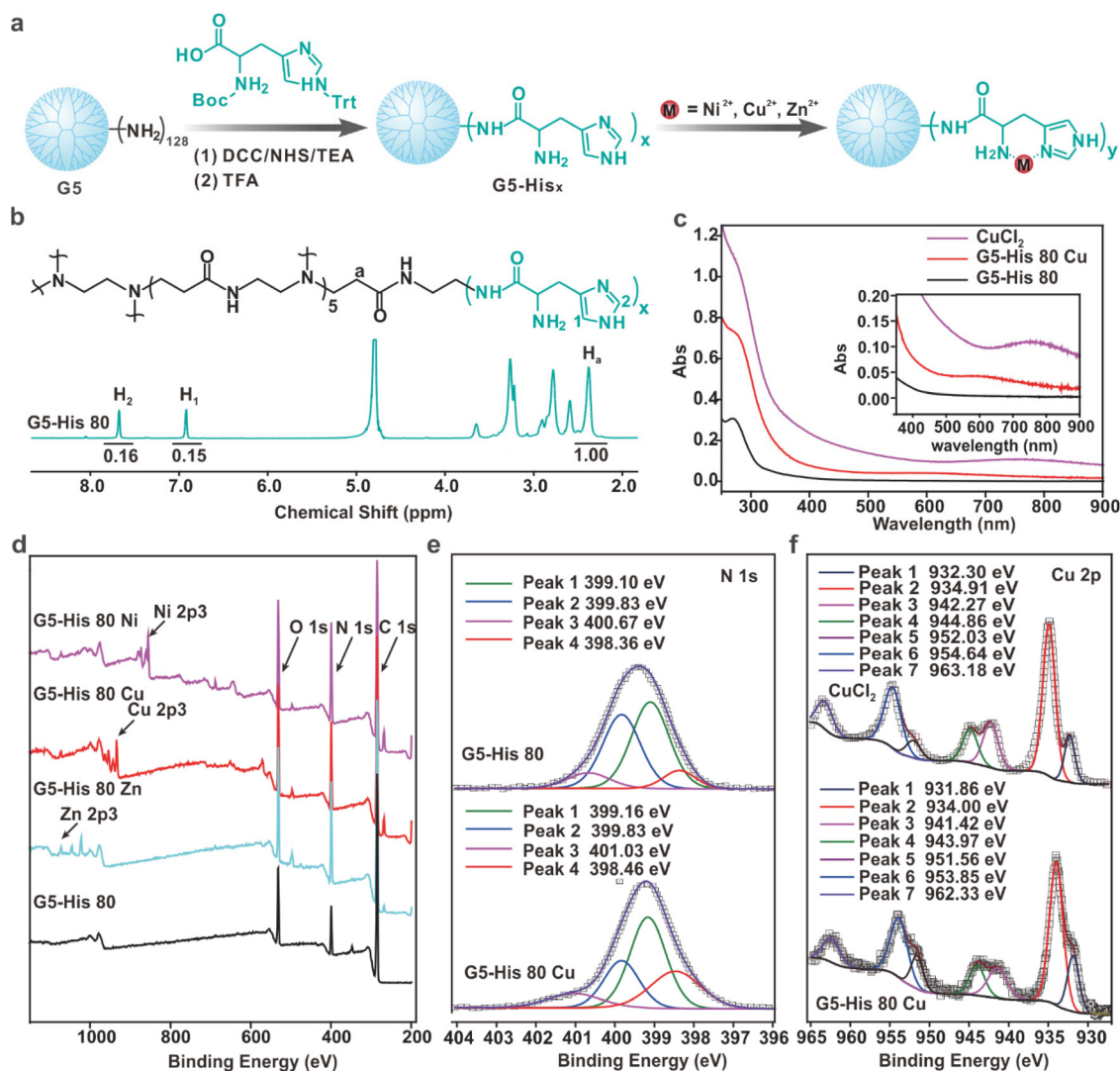
Fig. 1 Synthesis and characterization of the coordinative polymers. (a) Preparation of the coordinative polymers. (b) ^1\text{H} NMR spectrum of G5-His 80 in D 2 O. (c) UV-Vis spectra of \text{CuCl}_2 , G5-His 80 Cu, and G5-His 80 in aqueous solution. (d) XPS spectra of G5-His 80 Ni, G5-His 80 Cu, G5-His 80 Zn, and G5-His 80. (e) Magnified XPS N 1s spectra of G5-His 80 and G5-His 80 Cu. (f) Magnified XPS Cu 2p spectra of \text{CuCl}_2 and G5-His 80 Cu.
