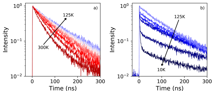
Fig. 6 (a) Temperature dependent X-ray excited decay spectra of PEA 2 PbBr 4 recorded from 125 K to 300 K, with a 25 K interval. The temperature decreases in the direction of the arrow. (b) Temperature dependent X-ray excited decay spectra of PEA 2 PbBr 4 recorded from 125 K to 25 K, with a 25 K interval, and at 10 K. The temperature decreases in the direction of the arrow.
