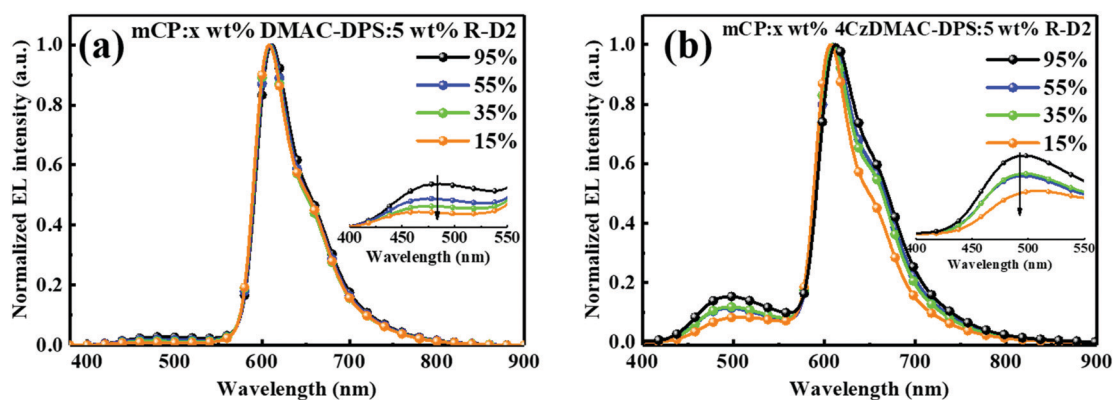
Fig. 5 Normalized EL spectra of (a) mCP:DMAC-DPS:R-D2 and (b) mCP:4CzDMAC-DPS:R-D2 doping systems. Inset: enlarged EL spectra from 400–550 nm.
