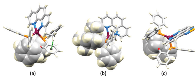
Fig. 14 (a) The structure of the [Cu(POP)(2-Etphen)] + cation in the [PF 6 ] - salt (CSD refcode PUTSAB) highlighting \pi -stacking within the POP ligand (space-filling representation) and Et...POP CH... \pi contact (hashed green line). (b) The structure of the [Cu(xantphos)(2-Etphen)] + cation in the [PF 6 ] - salt (CSD refcode PUTTAC) showing \pi -stacking within the xantphos ligand (space-filling representation, bottom of diagram) and accommodation of the Et group in the xanthene-bowl (space-filling, left). (c) The structure of the [Cu(POP)(5)] + cation in the [BF 4 ] - salt (CSD refcode PUYBET) with the \pi -stacking within the POP ligand shown in space-filling representation.
