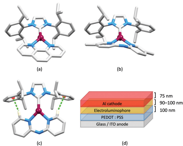
Fig. 24 Comparison of the structures of the [\text{Cu}(\text{N}^{\wedge}\text{N})(\text{NHC})]^+ cations in (a) [\text{Cu}(\text{phen})(\mathbf{42})][\text{BF}_4] (CSD refcode SORNOE) and (b) [\text{Cu}(5\text{-Mepy}_2\text{NH})(\mathbf{42})][\text{PF}_6] (refcode SORPIA). (c) Intramolecular \text{CH}\cdots\pi interactions in [\text{Cu}(\text{py}_2\text{NH})(\mathbf{42})][\text{PF}_6] (refcode SORPOG). (d) Architecture of the LECs containing Cu-iTMCs with NHC and \text{py}_2\text{NH} -type \text{N}^{\wedge}\text{N} ligands; LECs were driven using a pulsed current.
