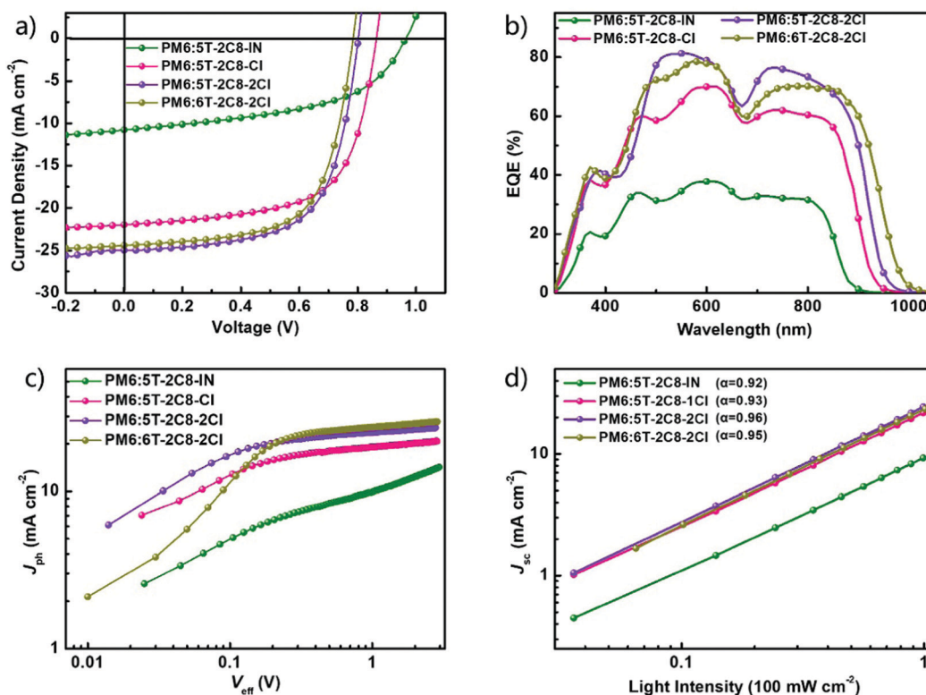
Fig. 2 (a) J - V curves of PM6:5T-2C8-IN/5T-2C8-Cl/5T-2C8-2Cl and PM6:6T-2C8-2Cl based devices under one sun illumination (AM 1.5G 100 mW cm -2 ). (b) EQE spectra of the corresponding devices. (c) J_{ph} versus V_{eff} and (d) light-intensity ( P ) dependence of J_{sc} measurement of the devices.
