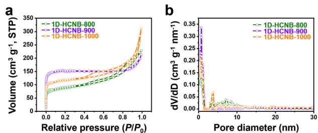
Fig. 4 (a) Nitrogen adsorption/desorption isotherms and (b) NLDFT pore size distribution curves of 1D-HCNB-800, 1D-HCNB-900, and 1D-HCNB-1000.
