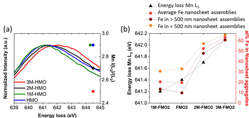
Fig. 8 (a) Left-Y Axis: EELS \text{Mn } L_3 peaks of HMO, 1M-HMO, 2M-HMO and 3M-HMO. Right-Y axis: corresponding \text{Mn } L_3/L_2 values. (b) Trends of oxidation state of x\text{M-HMO} (Left-Y axis) and Fe introduced by galvanic exchange reaction (right-Y axis) for x\text{M-FMO2} .
