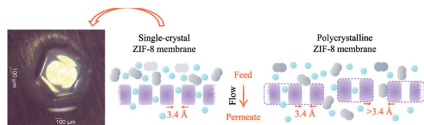
Fig. 7 Transport pathways through single crystal and polycrystalline ZIF-8 as membrane. Reprinted from C. Chen, A. Ozcan, A. O. Yazaydin and B. P. Ladewig, Gas permeation through single-crystal ZIF-8 membranes, Journal of Membrane Science , 2019, 575, 209–216, copyright (2019), with permission from Elsevier. 100
