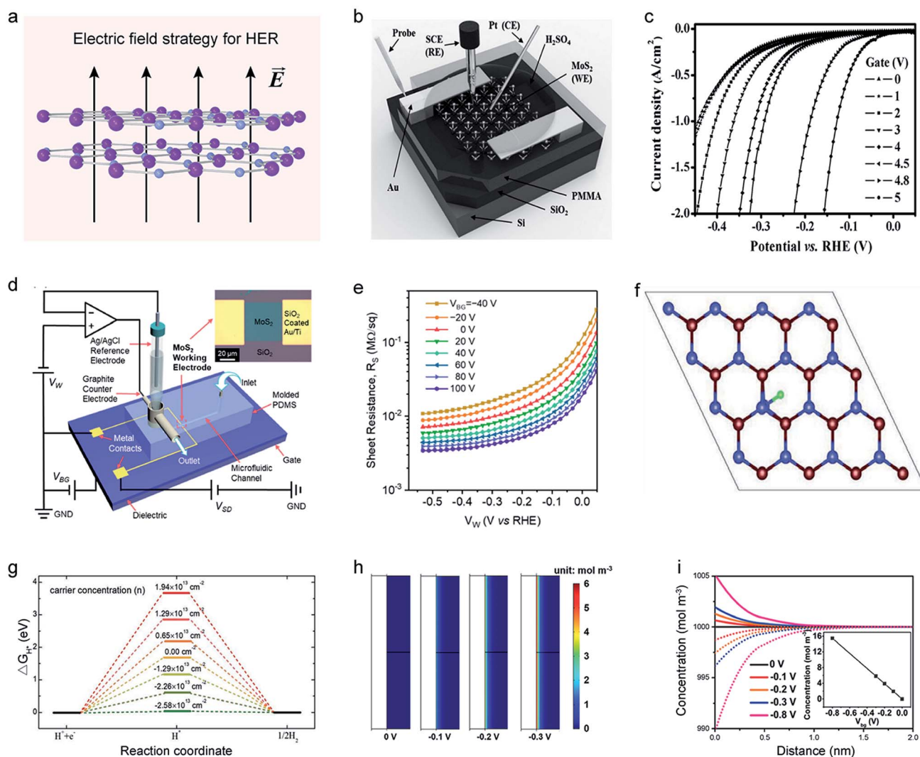
Fig. 10 Electric field strategy of 2D-TMDCs for HER. (a) Schematic illustration of the electric field strategy for HER. (b) Schematic illustration of a three-electrode microcell based on a \text{MoS}_2 nanosheet for HER measurement. (c) Polarization curves at varied back-gate voltages, as obtained from the micro-cell in (b). Reproduced with permission, 131 Wiley-VCH. (d) The structure of a back-gated microcell. Inset: the optical images of a \text{MoS}_2 -monolayer electrode. (e) The normalized sheet resistance of the \text{MoS}_2 electrode as a function of the electrode potential ( V_w ) at varied back-gate voltages ( V_{BG} ). Reproduced with permission, 135 American Chemical Society. (f) DFT calculation of an H-atom adsorbed on a \text{WSe}_2 nanosheet charged by the back-gate voltage (blue, purple, and green balls represent Se, W, and H atoms, respectively). (g) The Gibbs free-energy diagram of \text{WSe}_2 under different carrier concentrations. Reproduced with permission, 45 Wiley-VCH. (h) COMSOL simulation of the net charge distribution on the surface of a \text{VSe}_2 electrode at varied back-gate voltages. (i) Simulation results of charge concentrations on the surface (lines and dots represent \text{H}^+ and \text{SO}_4^{2-} , respectively). Inset: the net charge as a function of back-gate voltage. Reproduced with permission, 110 American Chemical Society.
