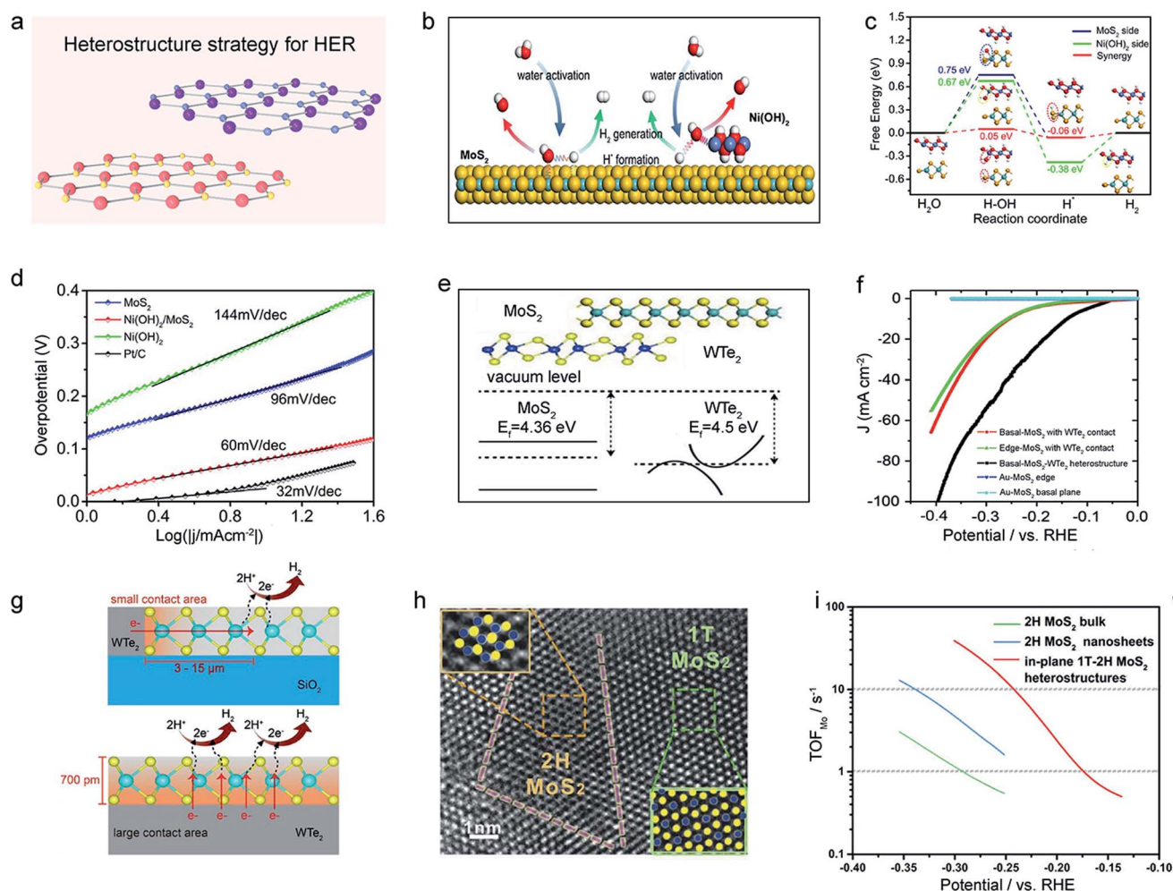
Fig. 13 Heterostructure strategy of 2D-TMDCs for HER. (a) Schematic illustration of the heterostructure strategy for HER. (b) Schematic illustration of the water activation process for the \text{Ni(OH)}_2/\text{MoS}_2 heterostructure in an alkaline solution. H, O, Mo, S, and Ni atoms are shown in white, red, cyan, yellow, and blue, respectively. The free energy diagram (c) and the Tafel plots (d) for \text{MoS}_2 , \text{Ni(OH)}_2 , and \text{Ni(OH)}_2/\text{MoS}_2 . Reproduced with permission, 188 Elsevier. (e) The aligned band structure of the \text{MoS}_2/\text{WTe}_2 heterostructure. (f) The corresponding polarization curves of the \text{MoS}_2/\text{WTe}_2 heterostructure. (g) Comparison of the HER mechanisms of the \text{MoS}_2/\text{WTe}_2 heterostructure (bottom) and \text{MoS}_2 with \text{WTe}_2 edge-contact (top). Reproduced with permission, 189 Wiley-VCH. HRTEM image (h) and the TOF (i) of the in-plane 1T-2H \text{MoS}_2 heterostructure. Reproduced with permission, 125 Wiley-VCH.
