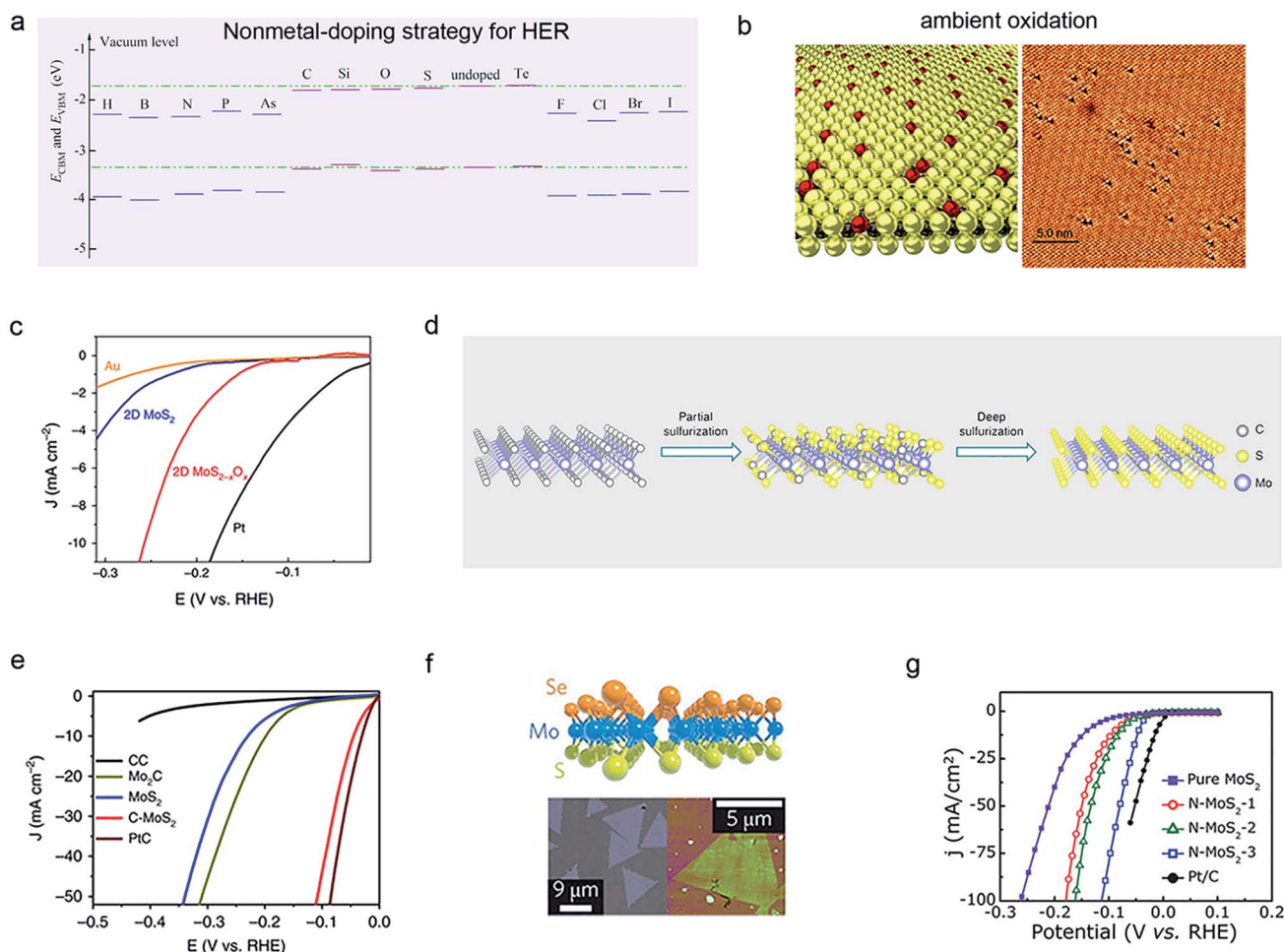
Fig. 5 Nonmetal-doping strategy of 2D-TMDCs for HER. (a) The calculated E_{\text{CBM}} and E_{\text{VBM}} of pristine and nonmetal-doped \text{MoSe}_2 monolayers. Reproduced with permission, 76 Springer Nature. (b) Atomic structure (left) and scanning tunneling microscopy (STM) images (right) of the exfoliated \text{MoS}_2 monolayer in the air after one month, and its corresponding HER performance (c). Reproduced with permission, 77 Springer Nature. Schematic illustration of carbon (C)-doped \text{MoS}_2 (d) and its corresponding HER performance in an alkaline electrolyte (e). Reproduced with permission, 79 Springer Nature. (f) Janus \text{MoS}_2 monolayer synthesized through a plasma-enhanced CVD method. Reproduced with permission, 81 Springer Nature. (g) Polarization curves of nitrogen (N)-doped \text{MoS}_2 samples. Reproduced with permission, 75 Wiley-VCH.
