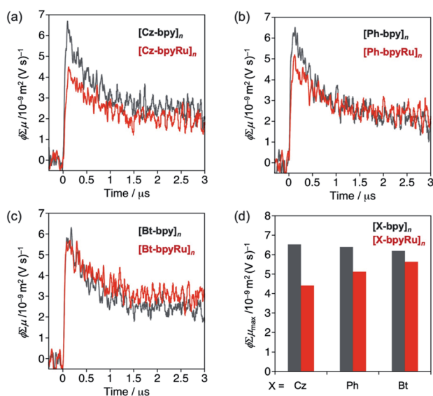
Fig. 3 Transient conductivities of (a) [\text{Cz-bpyM}]_n , (b) [\text{Ph-bpyM}]_n , and (c) [\text{Bt-bpyM}]_n ( \text{M} = \text{none} (grey) or \text{Ru} (red)), along with (d) their maximum values ( \phi\Sigma\mu_{\text{max}} ) obtained by photoexcitation at \lambda = 355 nm.
