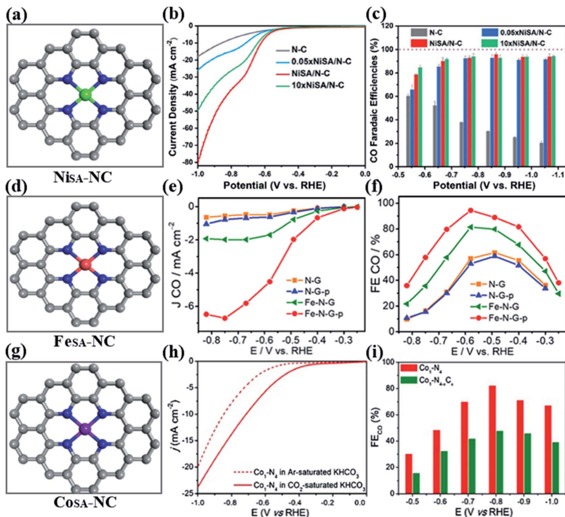
Fig. 2 (a) Structural model of \text{Ni}_{5\text{A}}\text{-NC} SACs. (b) Linear sweep voltammetry (LSV) curves at a scan rate of 10 \text{ mV s}^{-1} . (c) \text{FE}_{\text{CO}} for N-C, 0.05\text{xNi}_{5\text{A}}/\text{N-C} , \text{Ni}_{5\text{A}}/\text{N-C} , and 10\text{xNi}_{5\text{A}}/\text{N-C} catalysts tested in \text{CO}_2 -saturated 0.1 \text{ M KHCO}_3 electrolytes. Reproduced with permission from ref. 53. Copyright 2020, Elsevier. (d) Structural model of \text{Fe}_{5\text{A}}\text{-NC} SACs. (e) \text{CO} partial current density. (f) \text{FE}_{\text{CO}} for N-G, N-G-p, Fe-N-G, and Fe-N-G-p. Reproduced with permission from ref. 55. Copyright 2020, American Chemical Society. (g) Structural model of \text{Co}_{5\text{A}}\text{-NC} SACs. (h) LSV curves of \text{Co}_1\text{-N}_4 were recorded in \text{CO}_2 -saturated and Ar-saturated 0.1 \text{ M KHCO}_3 ( \text{pH} = 6.8 ) electrolytes. (i) \text{FE}_{\text{CO}} at selected potentials on \text{Co}_1\text{-N}_4 and \text{Co}_1\text{-N}_{4-x}\text{C}_x . Reproduced with permission from ref. 56. Copyright 2019, Elsevier.
