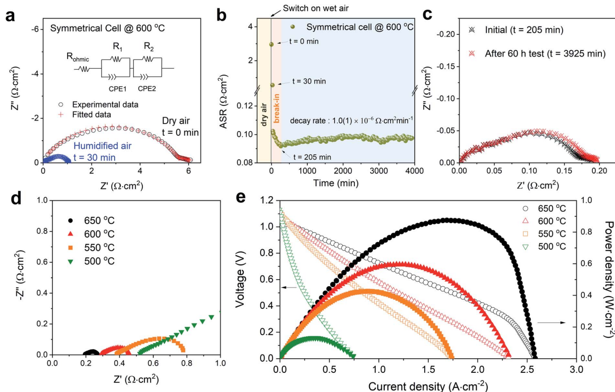
Fig. 3 (a) Impedance spectra (real vs. imaginary impedance) of a BSCFW|BZCYYb|BSCFW symmetrical cell under dry (black data points) and humidified 3 vol% \text{H}_2\text{O} -containing air (blue datapoints) conditions at 600 °C. The ohmic resistance ( R_{\text{ohmic}} ) including the contribution from the instrument and electrolyte is subtracted (the original impedance data is shown in Fig. S8†). The ASR of the cathode material is determined by the total resistance which is the sum of R_1 and R_2 (shown in the equivalent circuit diagram). (b) ASR of the symmetrical cell in 3 vol% water-containing air showing a 205 min break-in period after which the ASR stabilised and increases with a decay rate of 1.0(1) \times 10^{-6} \Omega \text{ cm}^2 \text{ min}^{-1} . (c) Impedance spectra plot of the symmetrical cell in Fig. 3b t = 205 min (after break-in period) and after the 60 h test ( t = 3925 min). (d) Impedance spectra of the single cell (BSCFW|BZCYYb|NiO-BZCYYb) measured under open-circuit condition, A reduced scale is displayed to show detail at higher temperature (full-scale plot is shown in Fig. S9†). (e) I - V curve (open symbols) and corresponding power density curves (filled symbols) of the BSCFW-BZCYYb single cell in the 500–650 °C temperature range.
