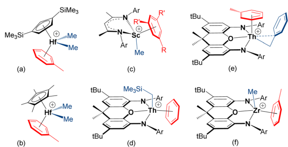
Fig. 1 Crystallographically-characterized early transition metal and f-element alkyl cations which exist as arene-solvent-separated ion pairs (R = Me or Br and R' = H, or R = R' = Me; Ar = C 6 H 3 1 Pr 2 -2,6 or C 6 H 2 1 Pr 3 -2,4,6). 8,10,13,14,18–20
