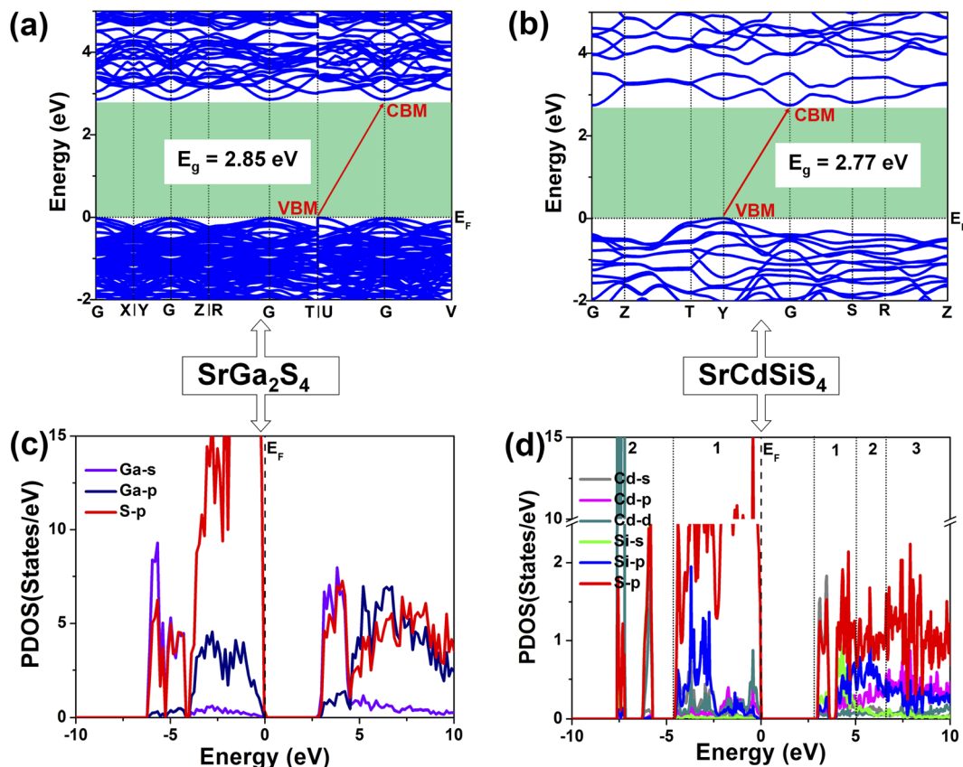
Fig. 5 Changes in (a and b) electronic band structures and (c and d) PDOSs (states with less contributions are omitted for better view) from \text{SrGa}_2\text{S}_4 to \text{SrCdSiS}_4 caused by dual-site aliovalent substitution.
