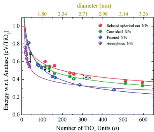
Fig. 7 The energy per \text{TiO}_2 unit with respect to bulk anatase (set to zero) of faceted (blue), annealed core-shell spherical (green), and amorphous (magenta) (\text{TiO}_2)_n nanoparticles as a function of n . An estimation of the diameter is reported via the upper x-axis. The black arrows indicate the energetic stabilisation of the (\text{TiO}_2)_{43} , (\text{TiO}_2)_{115} , and (\text{TiO}_2)_{136} core-shell nanoparticles upon annealing to nanoparticles with fully amorphized structures. Reproduced from ref. 42 with permission from the Royal Society of Chemistry.
