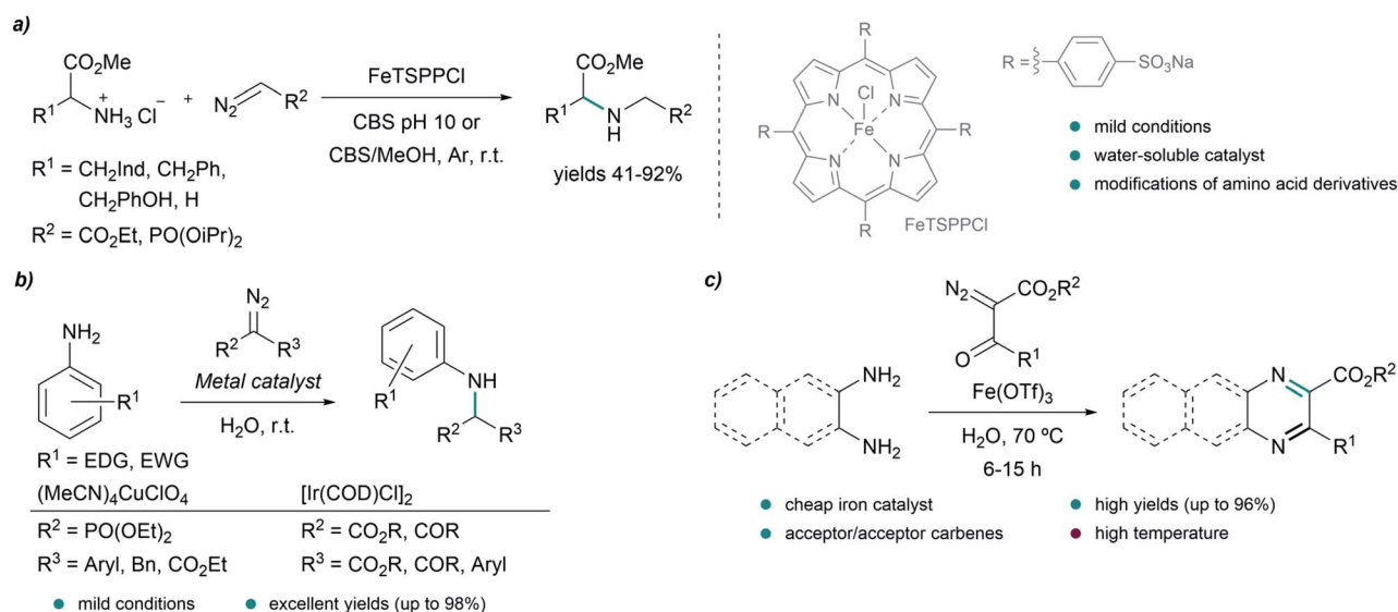
Fig. 5 N–H insertion reactions in water. (a) N–H insertion of iron carbenoids into amino acid derivatives catalyzed by a water soluble iron porphyrin in citrate buffer (CBS) reported by Simonneaux. (b) Carbene insertions into N–H bonds of anilines catalyzed by copper or iridium complexes reported by Sivasankar. (c) Iron catalyzed annulation of 1,2-diamines and diazodicarbonyl compounds reported by Lee.
